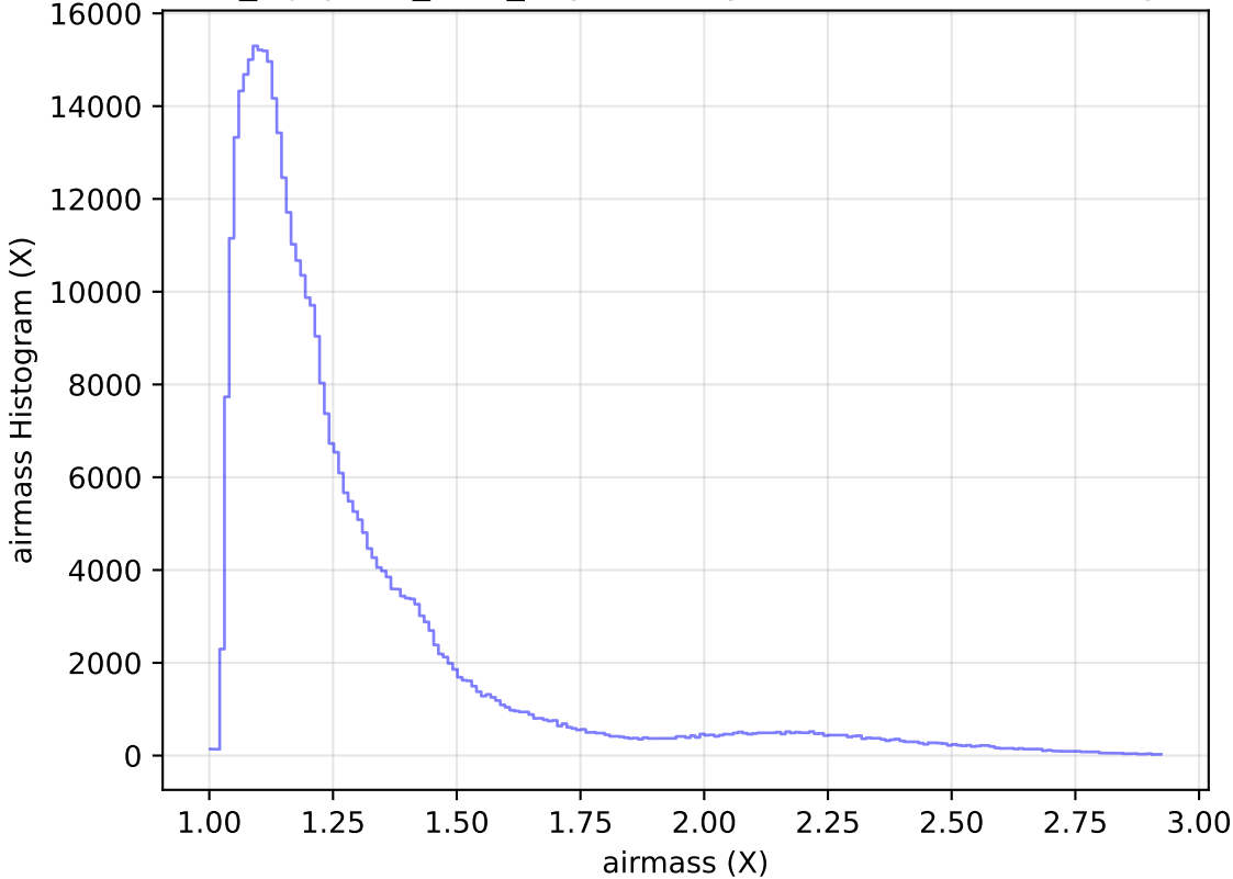
noroll_mjdp180_v3.4_10yrs All sky z band: airmass Histogram
