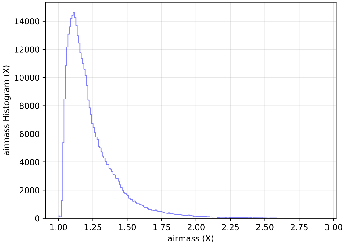
noroll_mjdp180_v3.4_10yrs All sky y band: airmass Histogram
