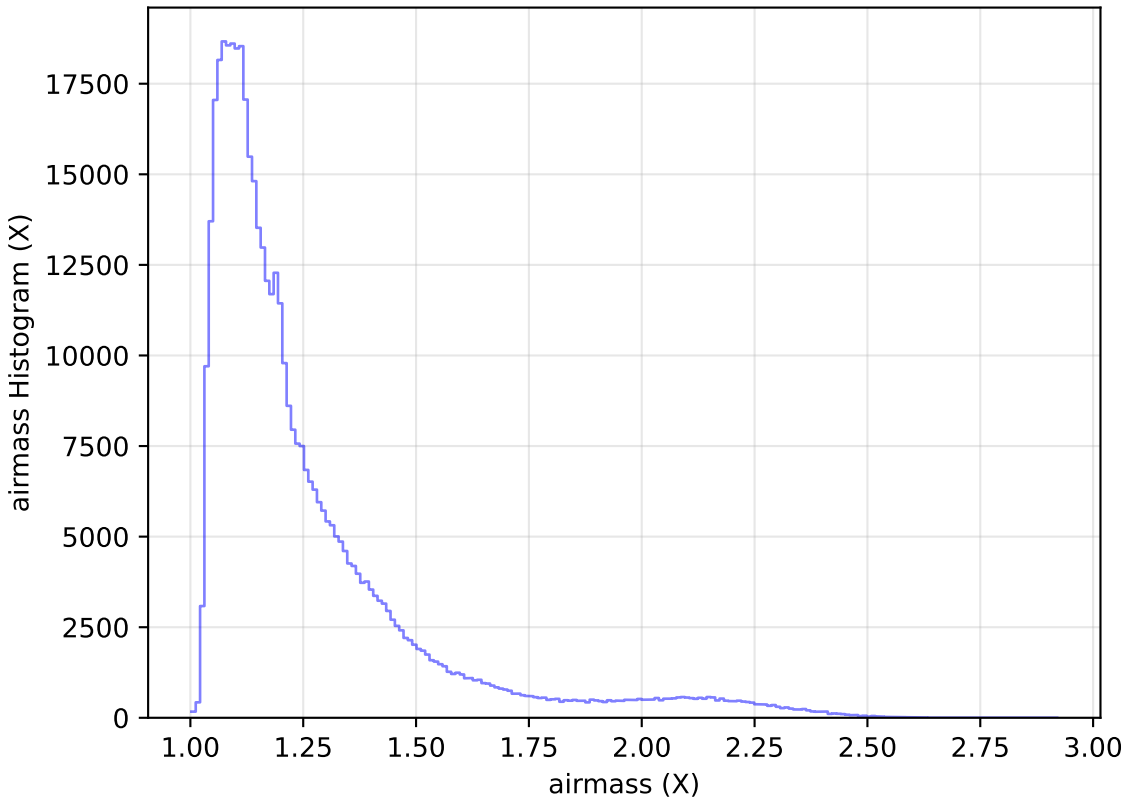
noroll_mjdp180_v3.4_10yrs All sky r band: airmass Histogram
