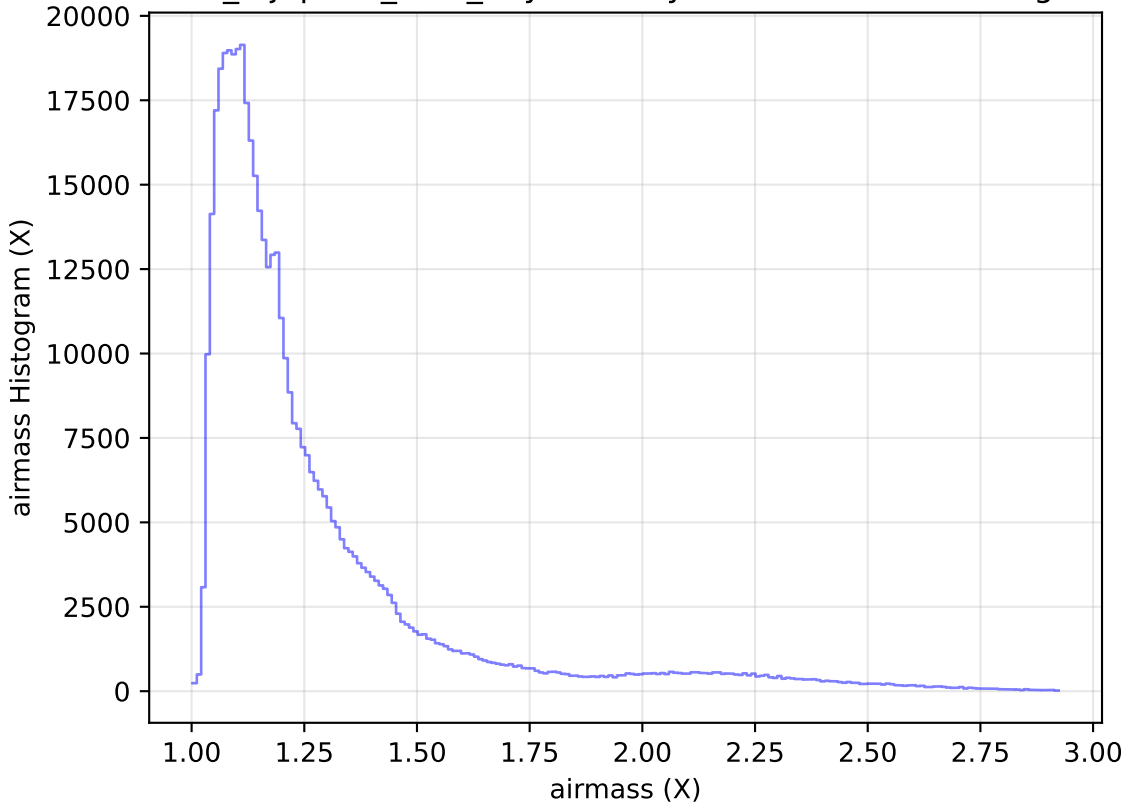
noroll_mjdp180_v3.4_10yrs All sky i band: airmass Histogram
