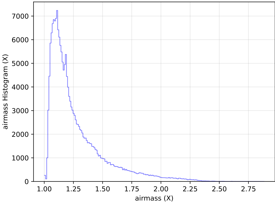
noroll_mjdp180_v3.4_10yrs All sky g band: airmass Histogram
