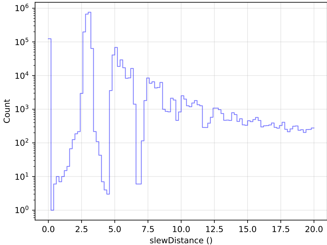
noroll_mjdp180_v3.4_10yrs All visits: Zoom Slew Distance Histogram
