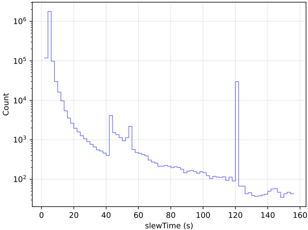
noroll_mjdp180_v3.4_10yrs All visits: Slew Time Histogram
