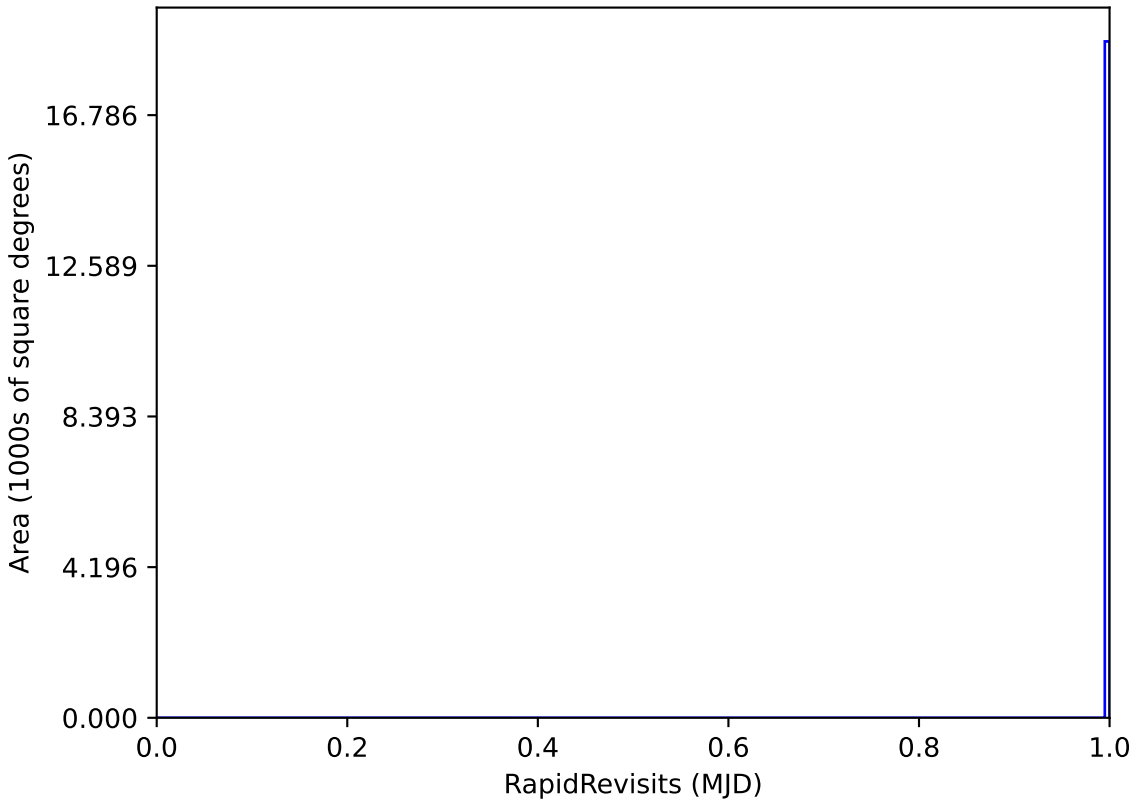
noroll_mjdp180_v3.4_10yrs WFD: RapidRevisits
