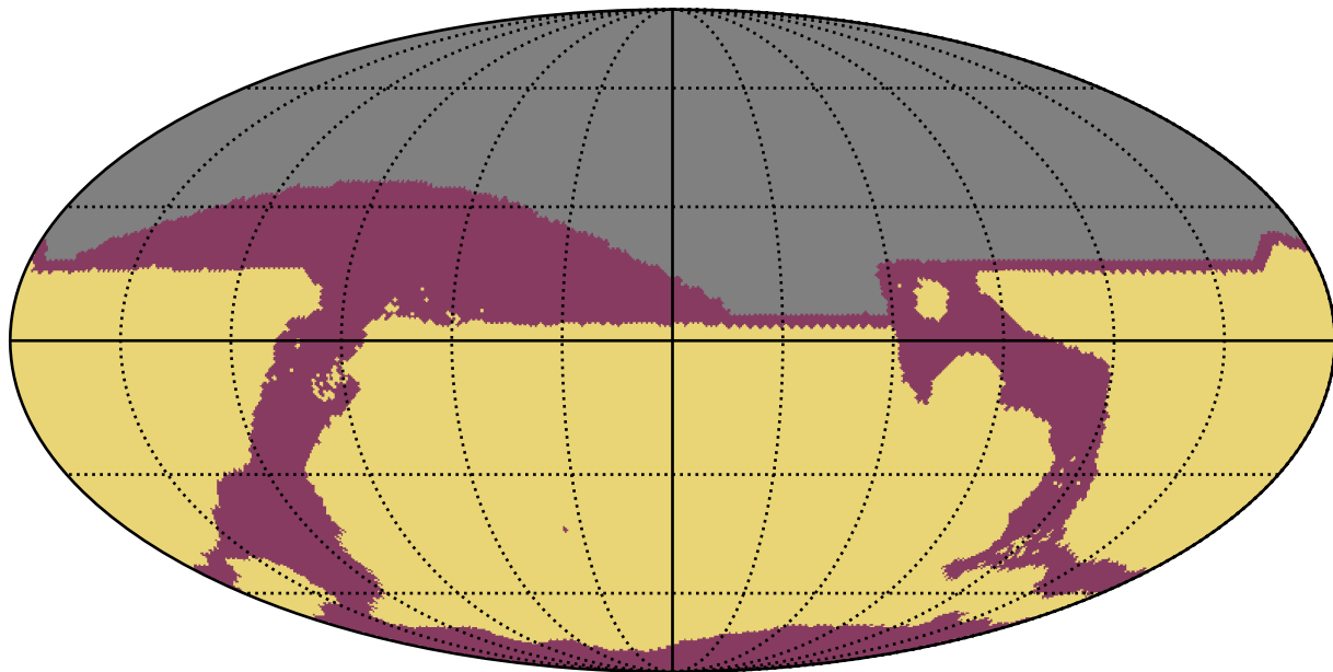
noroll_mjdp180_v3.4_10yrs All sky: RapidRevisits
