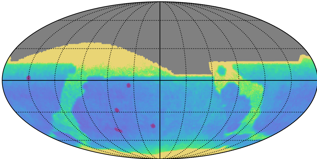
noroll_mjdp180_v3.4_10yrs All sky: Proper Motion Uncert @ 24.0
