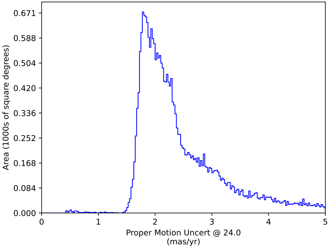
noroll_mjdp180_v3.4_10yrs All sky: Proper Motion Uncert @ 24.0
