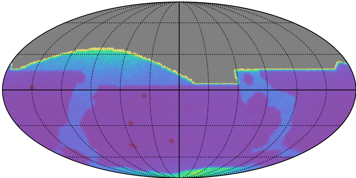
noroll_mjdp180_v3.4_10yrs All sky: Proper Motion Uncert @ 20.5
