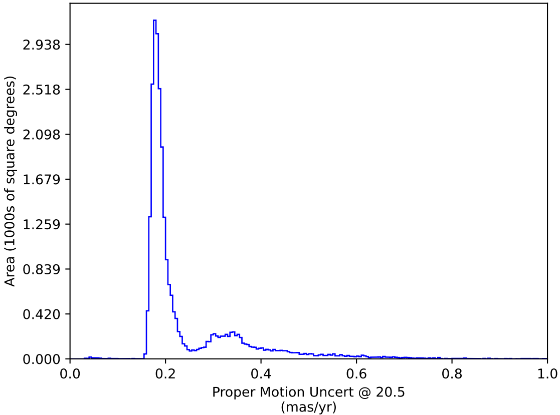
noroll_mjdp180_v3.4_10yrs All sky: Proper Motion Uncert @ 20.5
