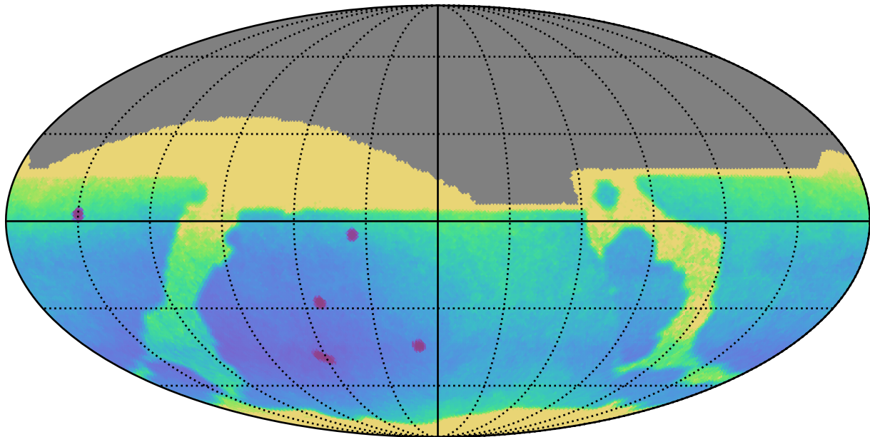
noroll_mjdp180_v3.4_10yrs All sky: Parallax Uncert @ 24.0
