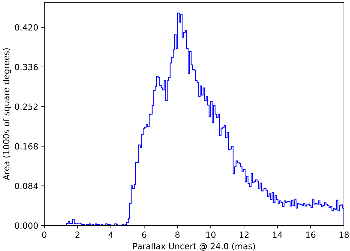
noroll_mjdp180_v3.4_10yrs All sky: Parallax Uncert @ 24.0
