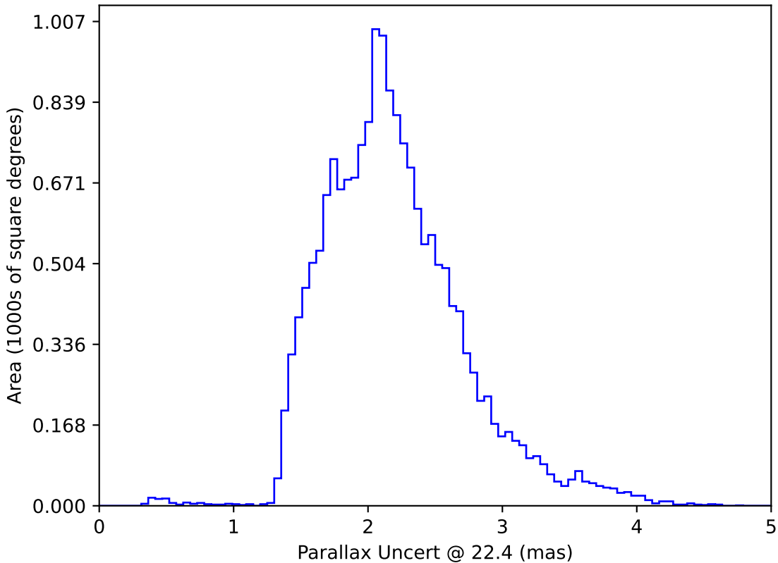
noroll_mjdp180_v3.4_10yrs WFD: Parallax Uncert @ 22.4
