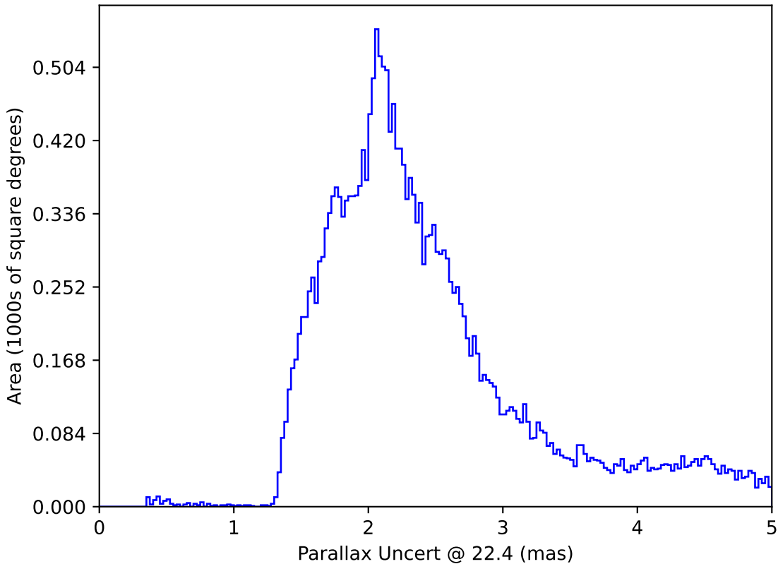
noroll_mjdp180_v3.4_10yrs All sky: Parallax Uncert @ 22.4
