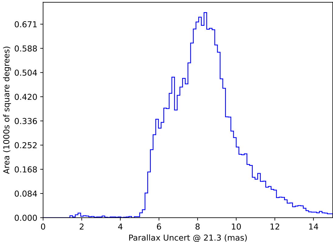
noroll_mjdp180_v3.4_10yrs WFD y band only: Parallax Uncert @ 21.3
