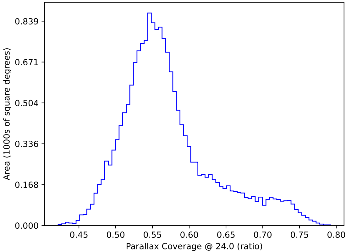
noroll_mjdp180_v3.4_10yrs WFD: Parallax Coverage @ 24.0
