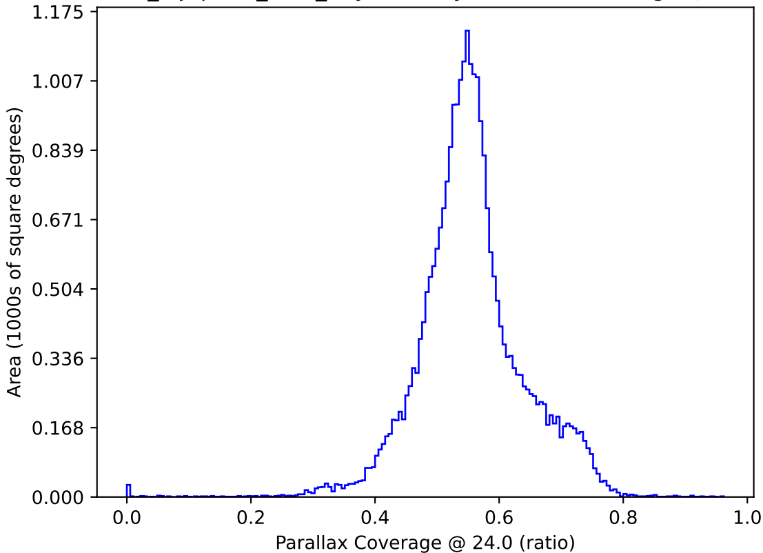
noroll_mjdp180_v3.4_10yrs All sky: Parallax Coverage @ 24.0
