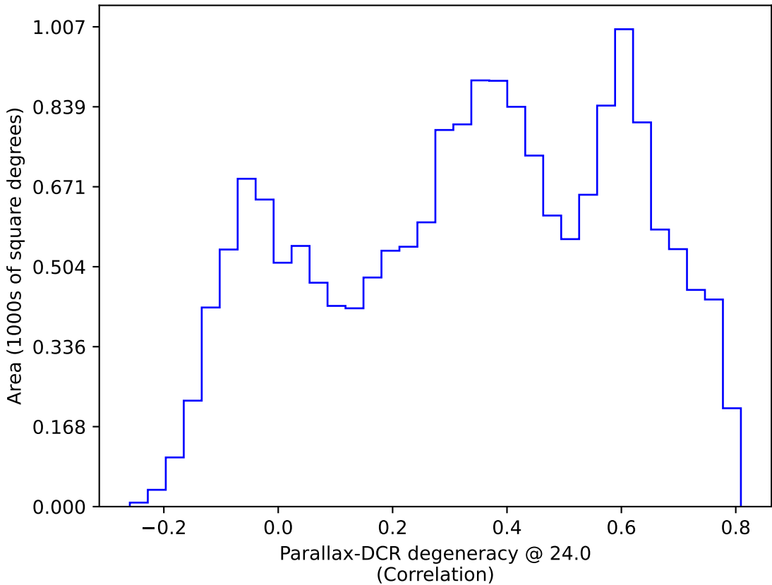
noroll_mjdp180_v3.4_10yrs WFD: Parallax-DCR degeneracy @ 24.0
