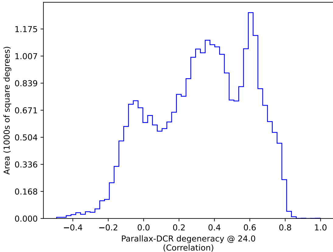
noroll_mjdp180_v3.4_10yrs All sky: Parallax-DCR degeneracy @ 24.0
