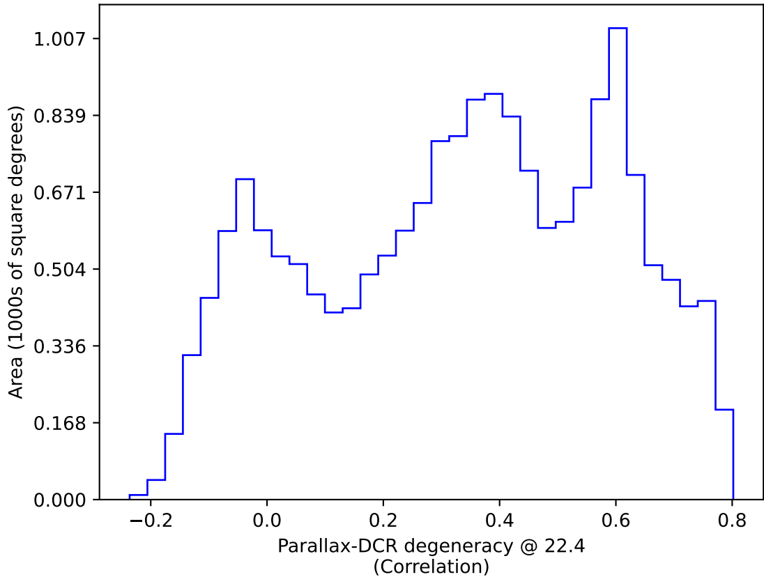
noroll_mjdp180_v3.4_10yrs WFD: Parallax-DCR degeneracy @ 22.4
