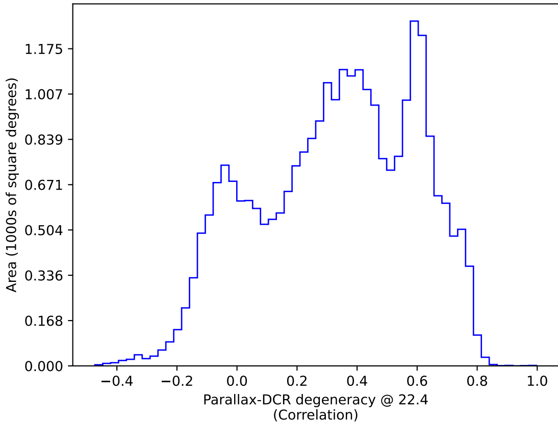
noroll_mjdp180_v3.4_10yrs All sky: Parallax-DCR degeneracy @ 22.4
