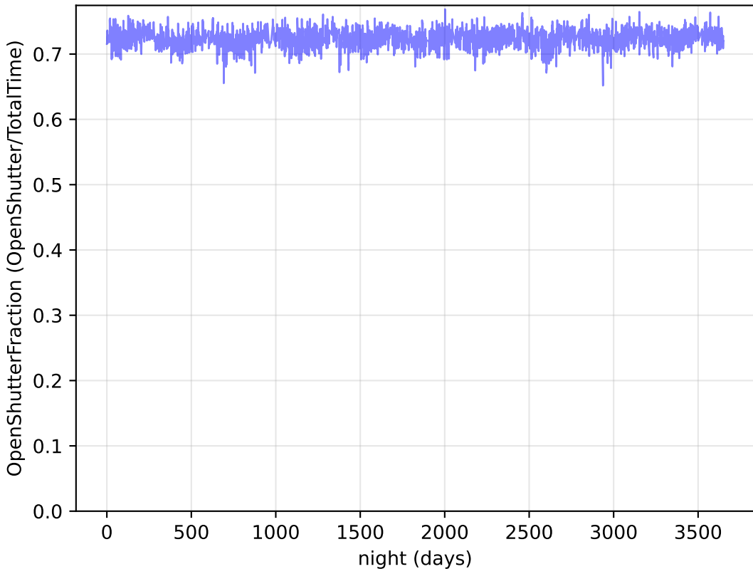
noroll_mjdp180_v3.4_10yrs Per night: OpenShutterFraction
