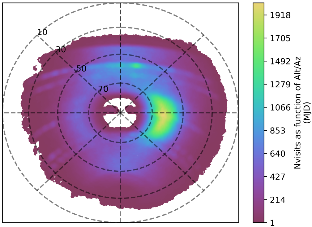
noroll_mjdp180_v3.4_10yrs y band: Nvisits as function of Alt/Az
