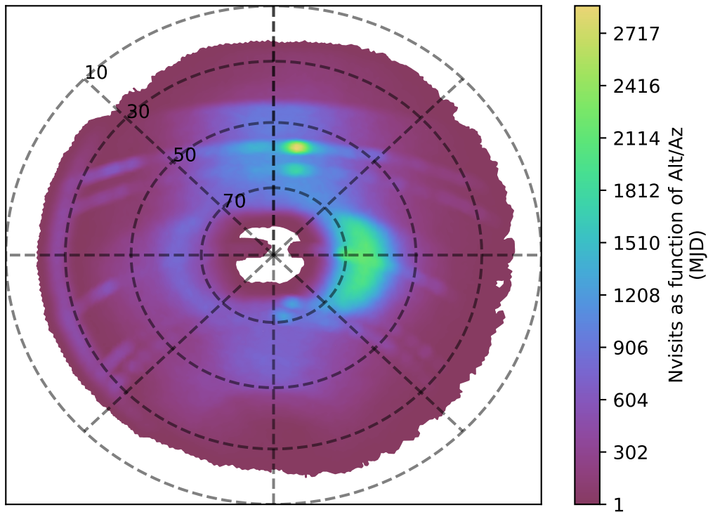
noroll_mjdp180_v3.4_10yrs r band: Nvisits as function of Alt/Az
