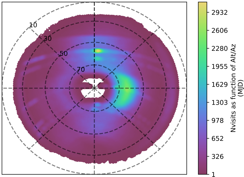
noroll_mjdp180_v3.4_10yrs i band: Nvisits as function of Alt/Az
