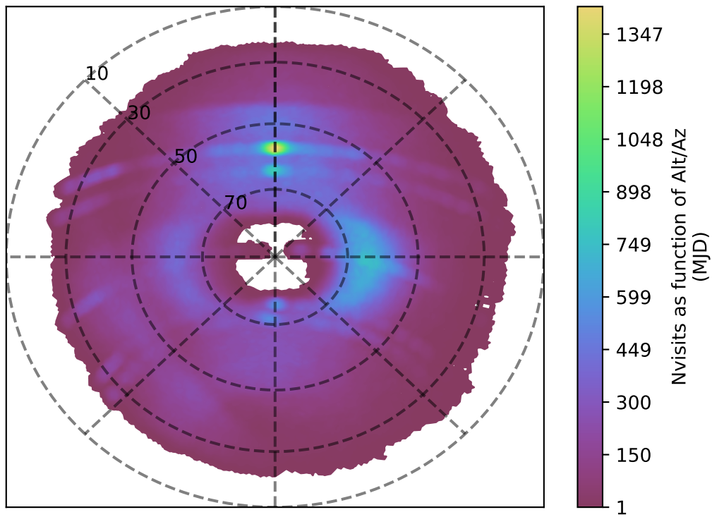
noroll_mjdp180_v3.4_10yrs g band: Nvisits as function of Alt/Az
