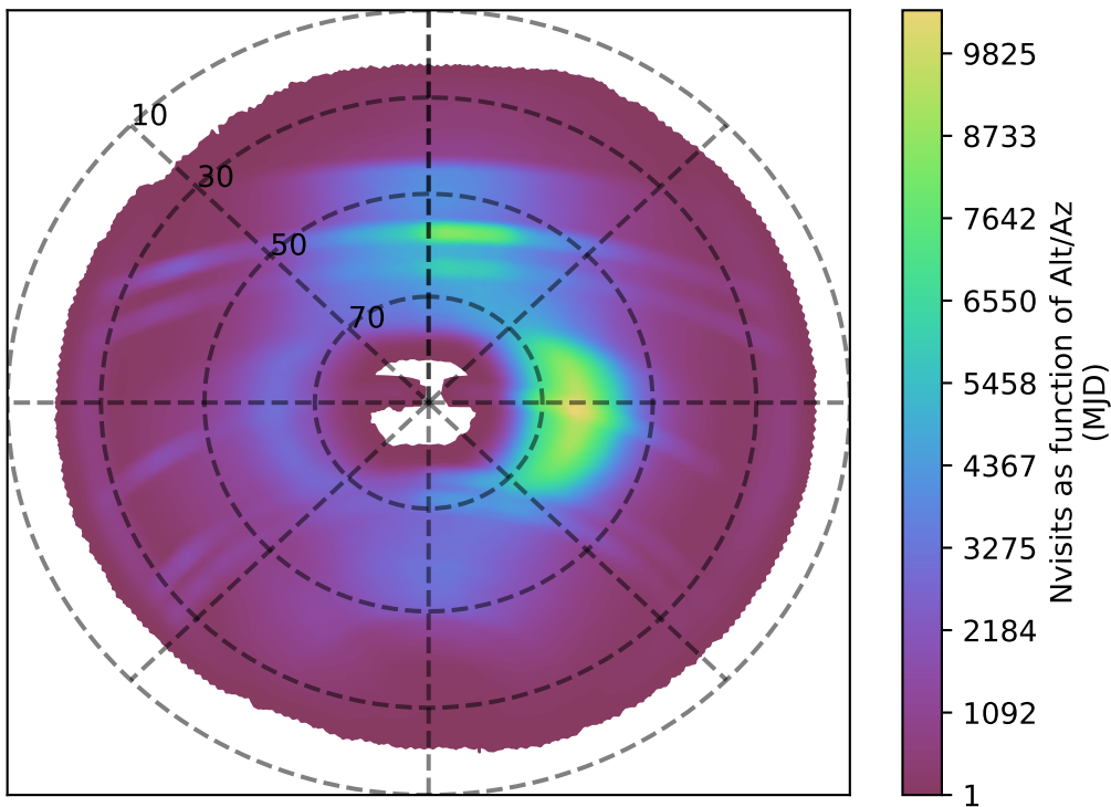
noroll_mjdp180_v3.4_10yrs all bands: Nvisits as function of Alt/Az
