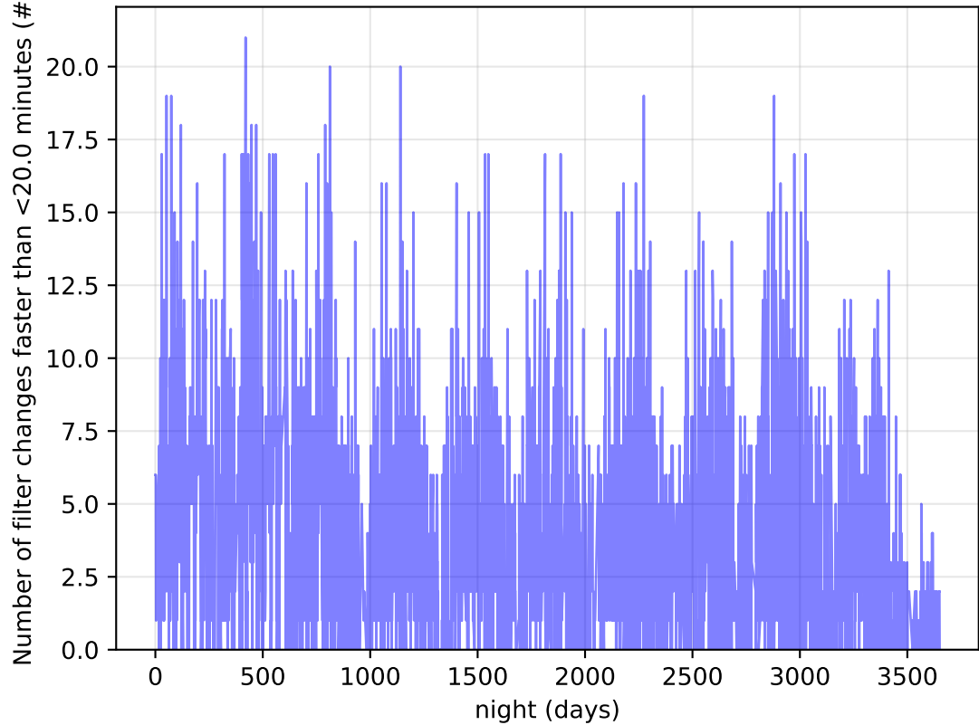
noroll_midp180_v3.4_10yrs Per Night: Number of filter changes faster than <20.0 minutes
