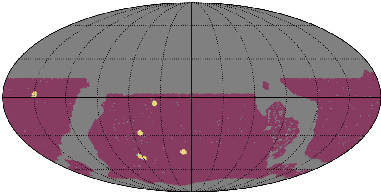
noroll_mjdp180_v3.4_10yrs WFD: NumberOfQuickRevisits
