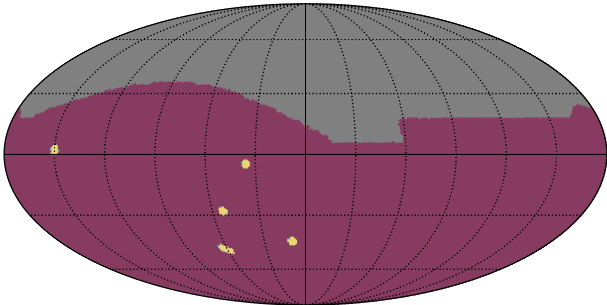
noroll_mjdp180_v3.4_10yrs All sky: NumberOfQuickRevisits
