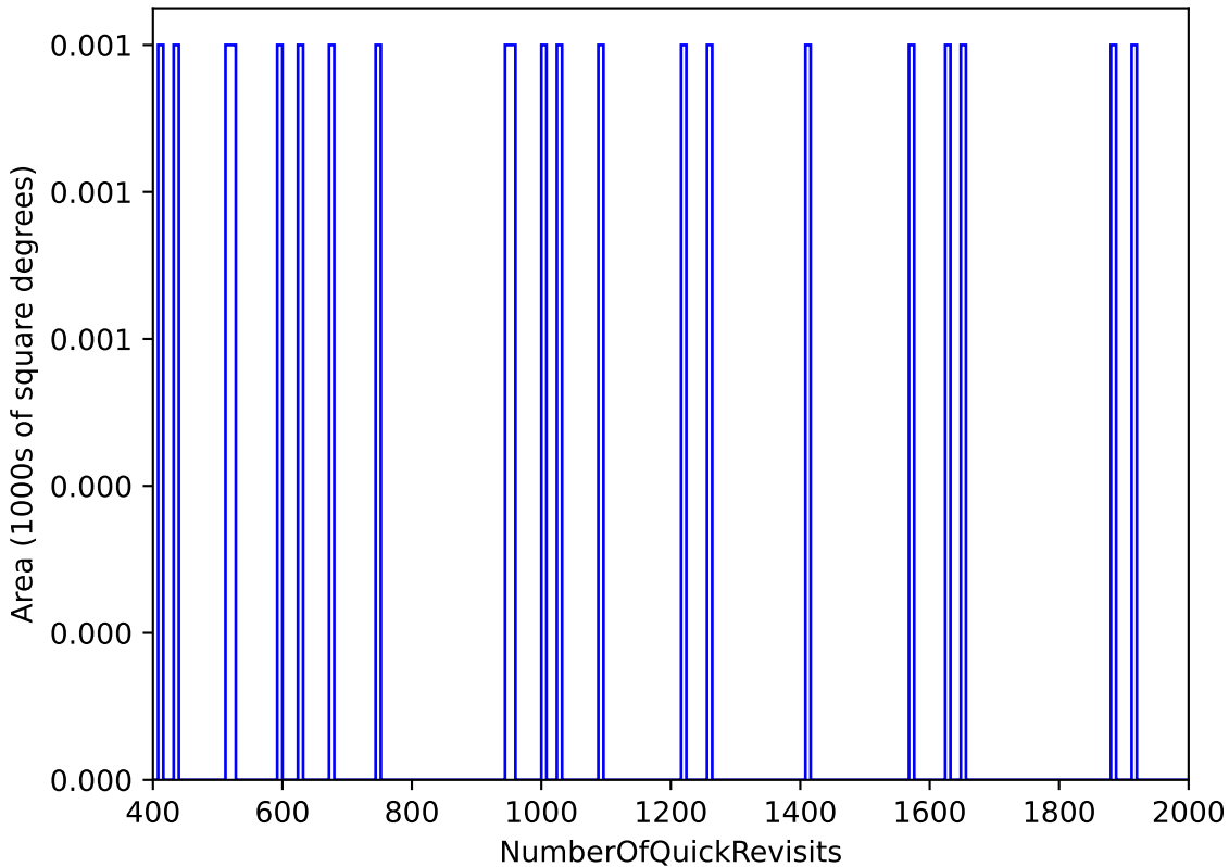
noroll_mjdp180_v3.4_10yrs All sky: NumberOfQuickRevisits
