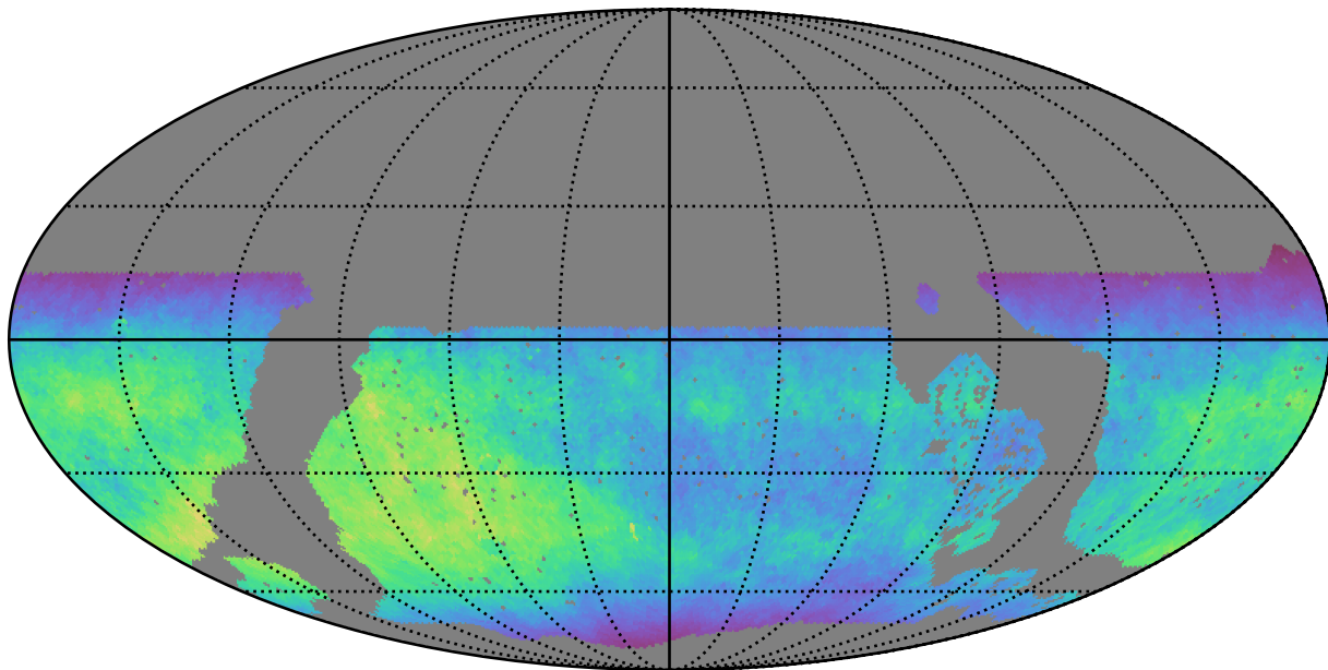
noroll_mjdp180_v3.4_10yrs WFD z band: Normalized Teff
