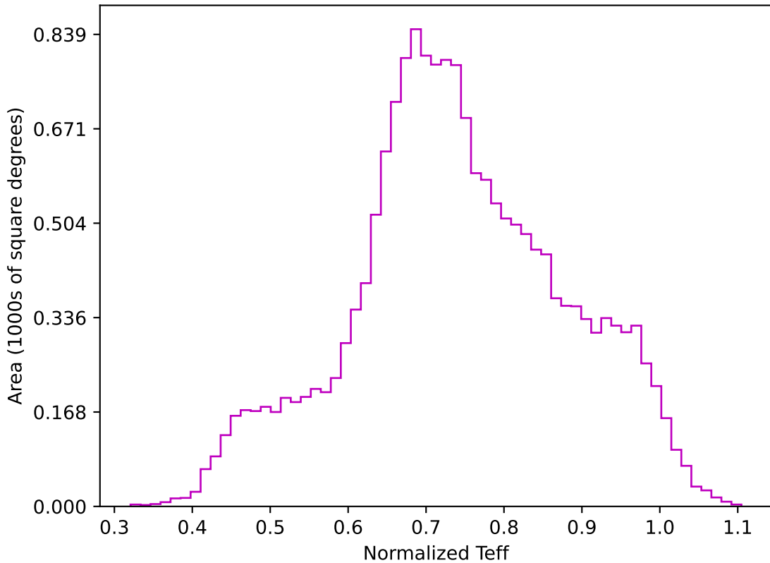
noroll_mjdp180_v3.4_10yrs WFD z band: Normalized Teff
