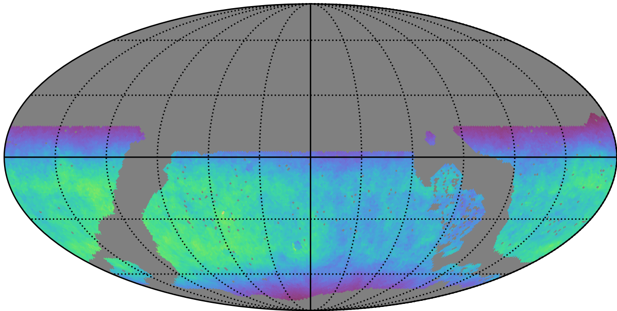
noroll_mjdp180_v3.4_10yrs WFD y band: Normalized Teff
