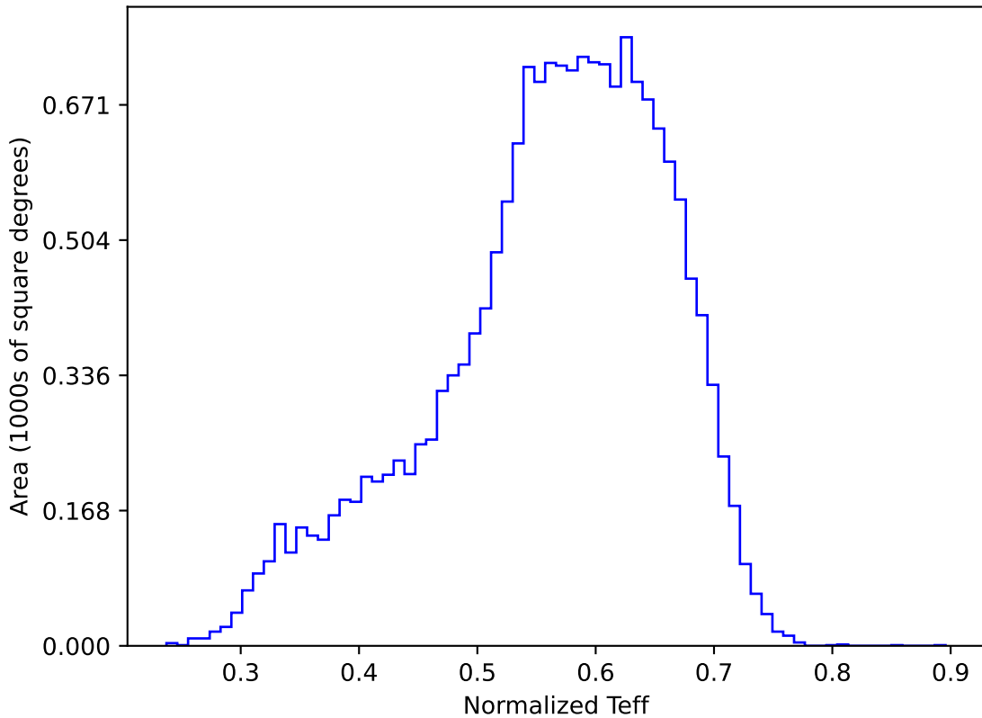
noroll_mjdp180_v3.4_10yrs WFD y band: Normalized Teff
