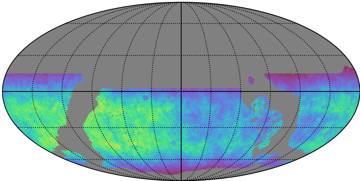
noroll_mjdp180_v3.4_10yrs WFD u band: Normalized Teff
