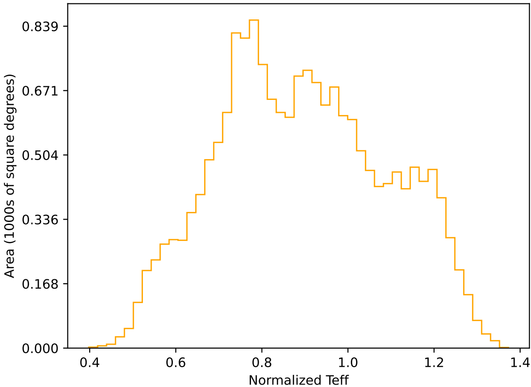
noroll_mjdp180_v3.4_10yrs WFD r band: Normalized Teff
