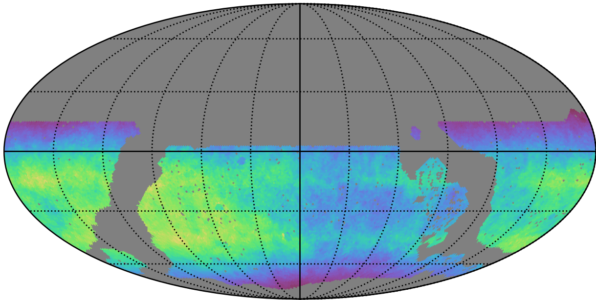
noroll_mjdp180_v3.4_10yrs WFD i band: Normalized Teff
