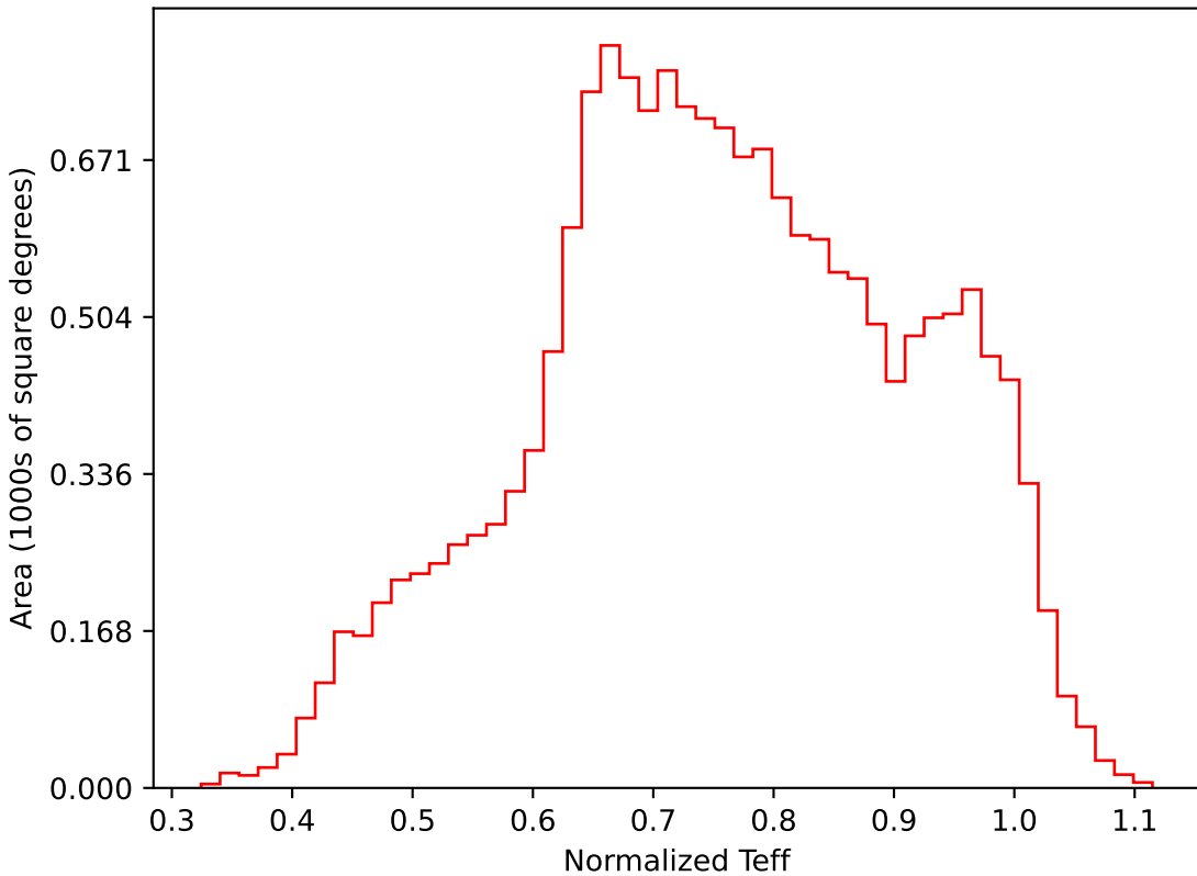
noroll_mjdp180_v3.4_10yrs WFD i band: Normalized Teff
