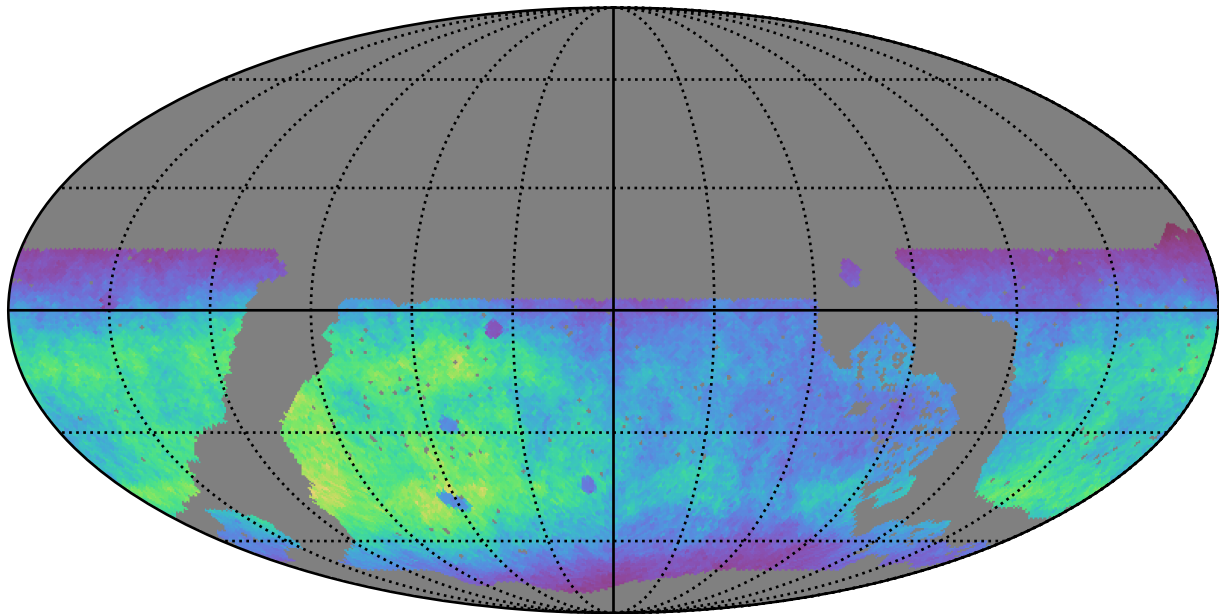
noroll_mjdp180_v3.4_10yrs WFD g band: Normalized Teff
