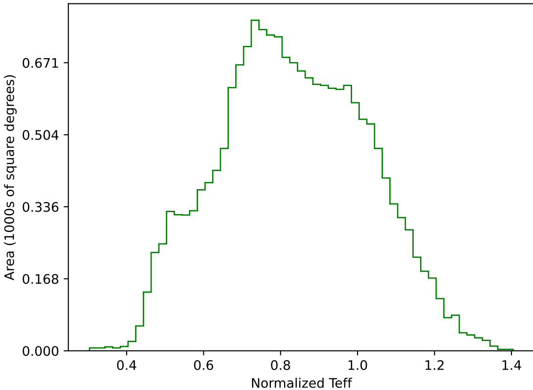
noroll_mjdp180_v3.4_10yrs WFD g band: Normalized Teff
