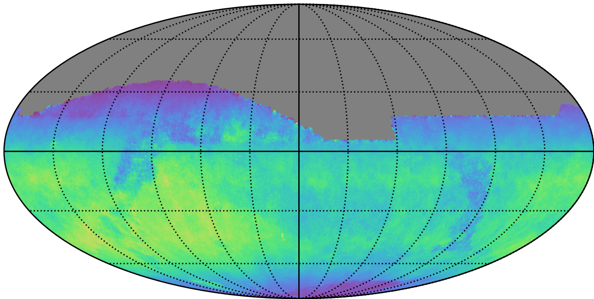
noroll_mjdp180_v3.4_10yrs All sky z band: Normalized Teff
