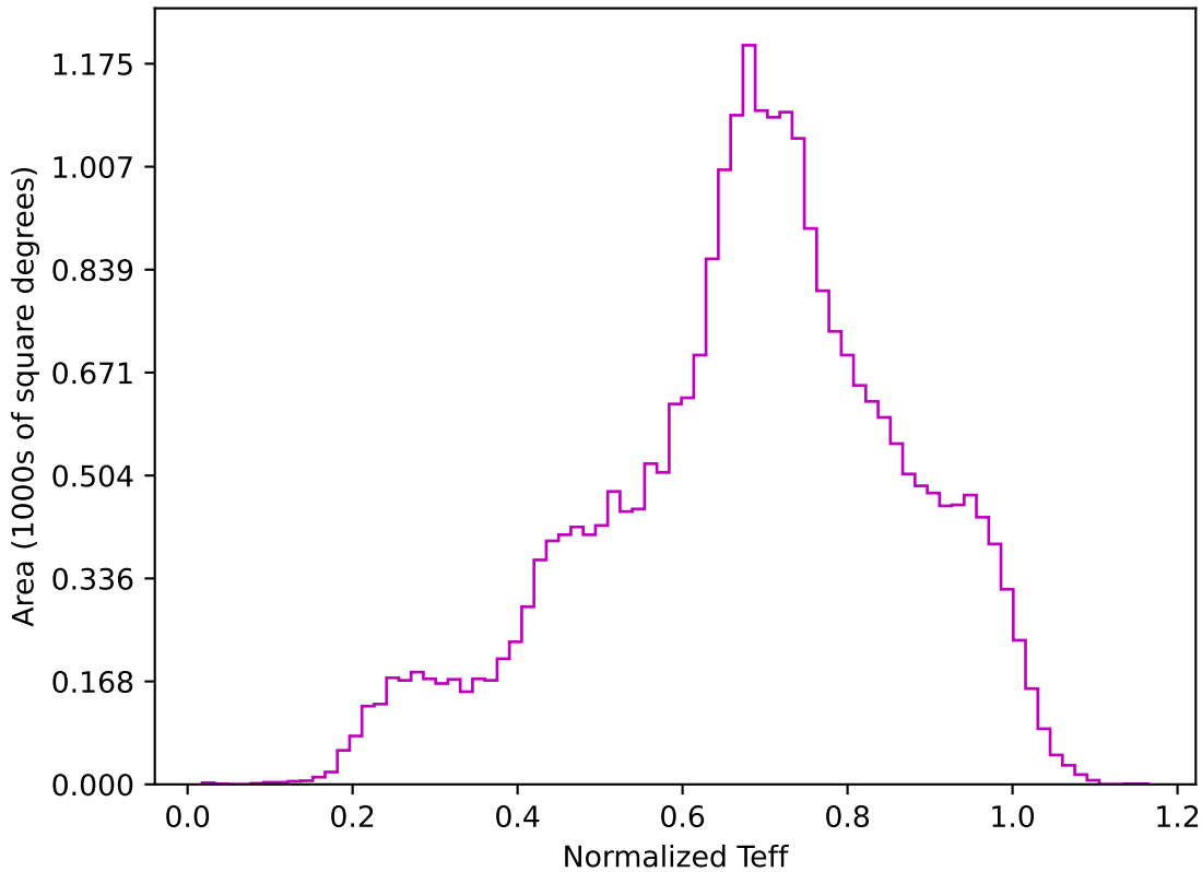
noroll_mjdp180_v3.4_10yrs All sky z band: Normalized Teff
