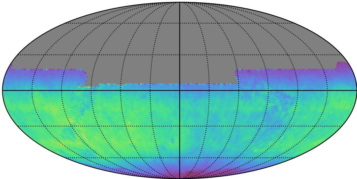
noroll_mjdp180_v3.4_10yrs All sky y band: Normalized Teff
