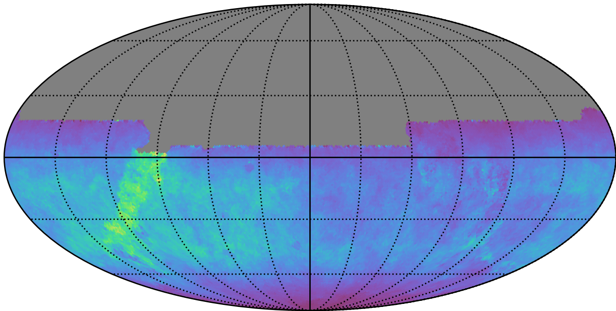
noroll_mjdp180_v3.4_10yrs All sky u band: Normalized Teff
