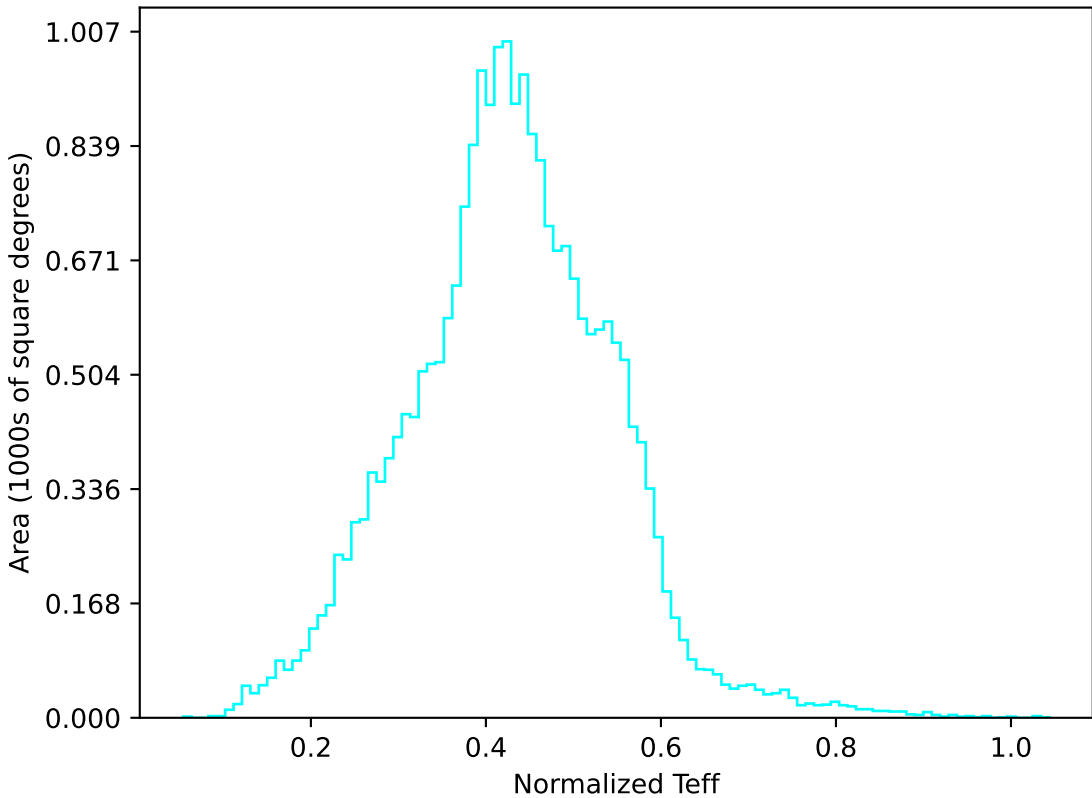
noroll_mjdp180_v3.4_10yrs All sky u band: Normalized Teff
