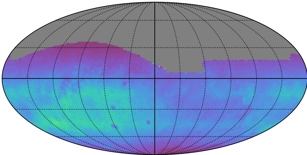
noroll_mjdp180_v3.4_10yrs All sky r band: Normalized Teff
